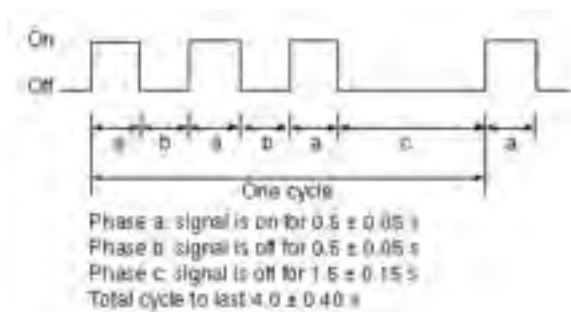
Figure A-3.2.4.20.(2).A. Temporal Pattern for Fire Alarm Signal
