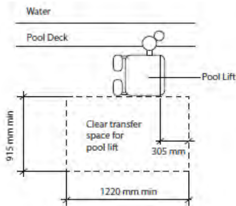
Figure A-3.11.3.3.(4) Transfer Space at Pool Lift
