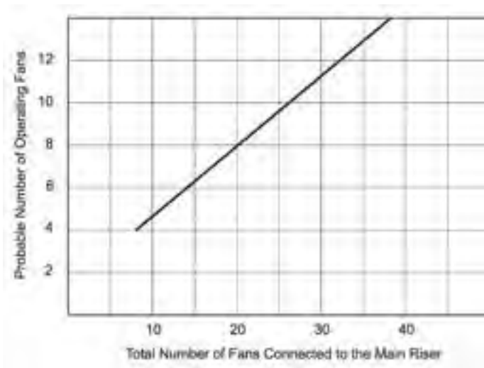
Figure A-6.2.3.8.(10)(b) Operation Diversity Factor
