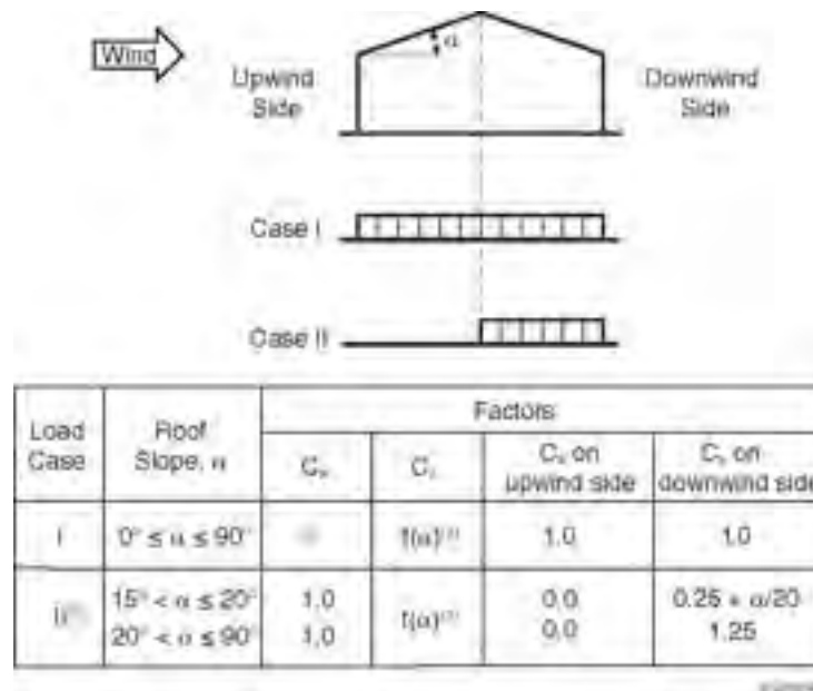
Figure A-4.1.6.9. Load Cases for Gable Roofs
