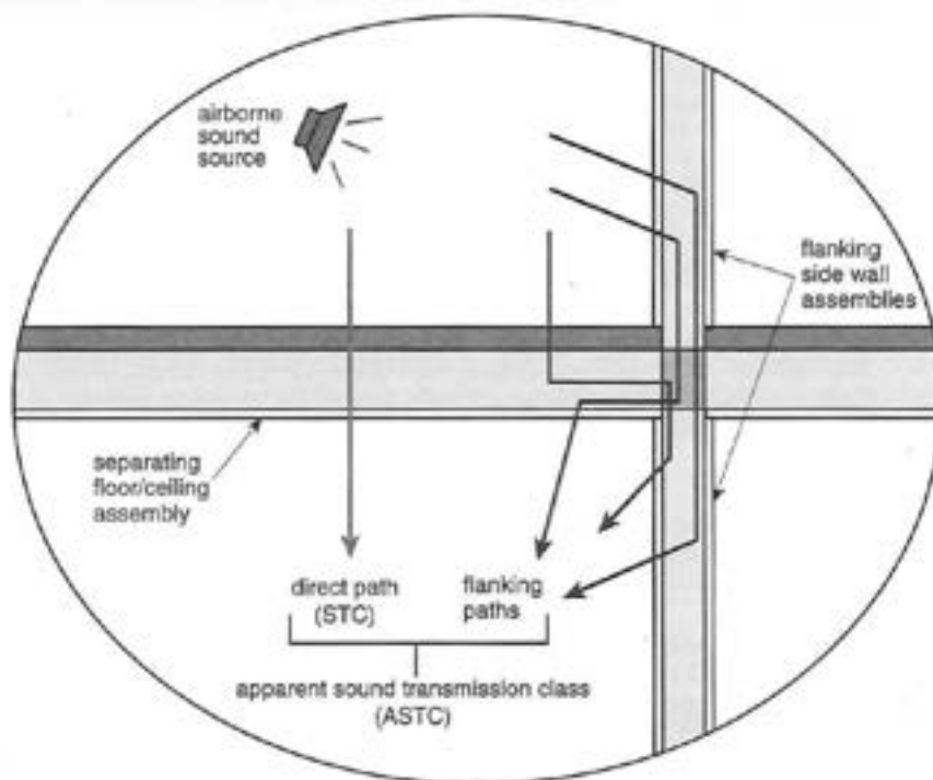
Figure A-9.11.B. Vertical Sound Transmission Paths Floor/Wall Junction
