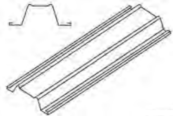
Figure 3 Example of Steel Furring Channel
