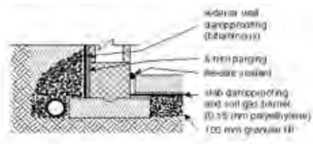
Figure SB-9B Dampproofing and Soil Gas Control at Foundation Wall/Floor Junctions with Hollow Walls
