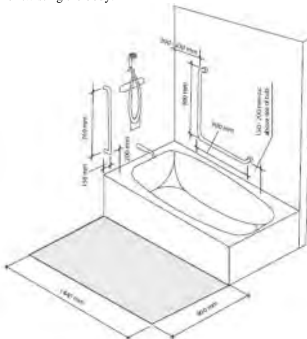
Figure A-3.8.3.13.(4) Bathtub
