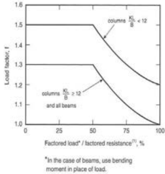
Figure 2.11.2.A. Factors to Compensate for Partially Loaded Columns and Beams
