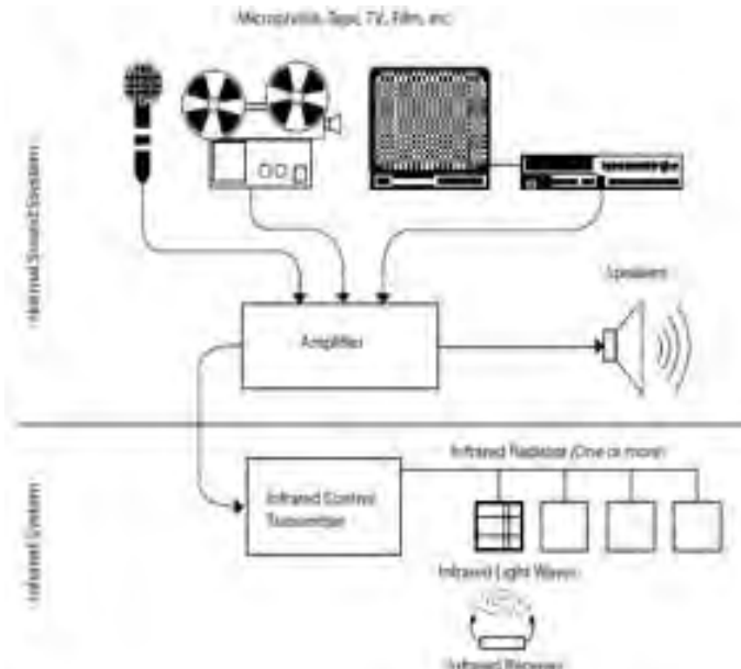
Figure A-3.8.3.7.(1)B Infrared Sound Transmission System
