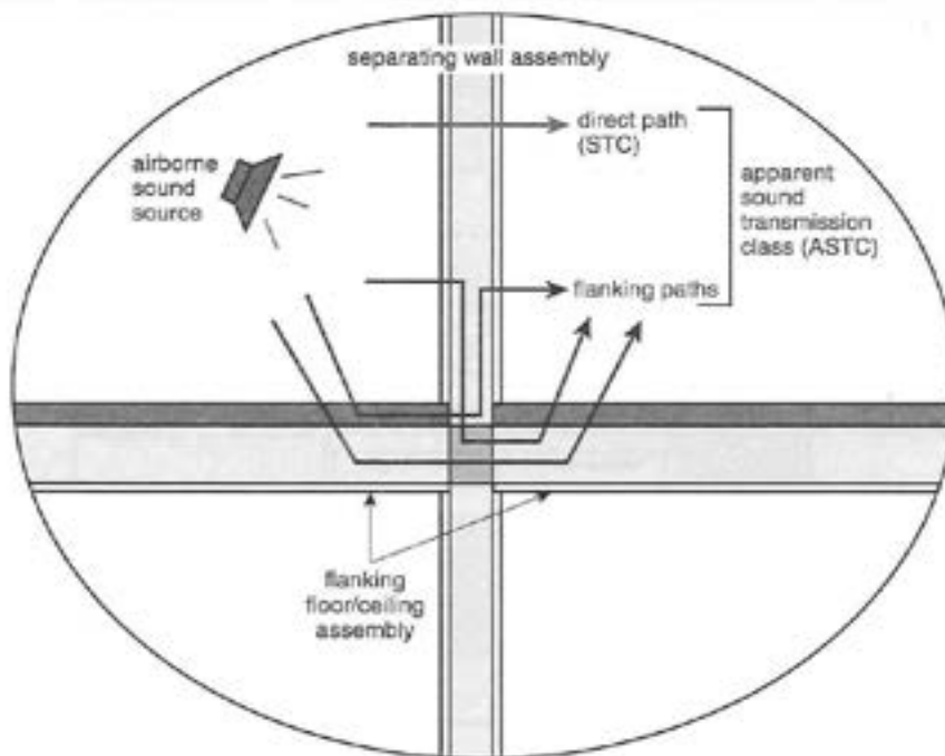
Figure A-9.11.A. Horizontal Sound Transmission Paths Floor/Wall Junction
