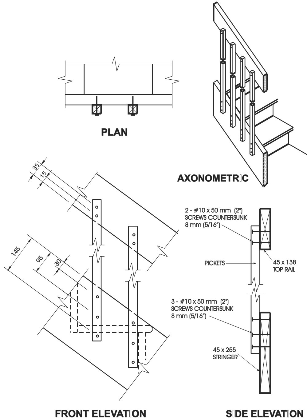
Detail IH-1
