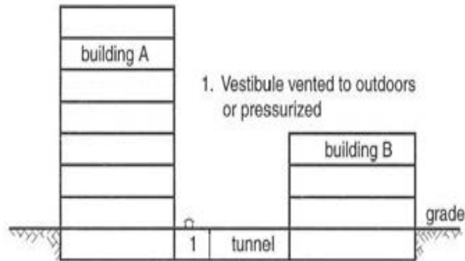
Figure 17 Section through buildings linked by underground tunnel
