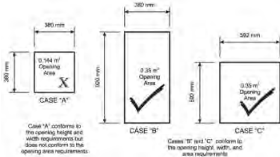
Figure A-9.9.10.1.(1) Window Opening Areas and Dimensions
