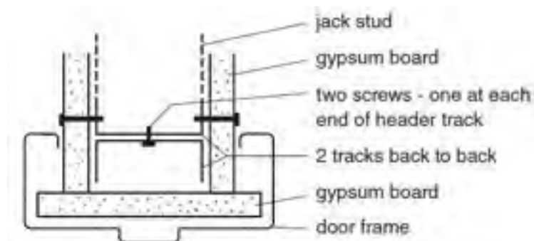
Figure A-9.24.3.2.(3) Steel Stud Header Detail
