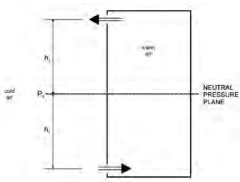
Figure B-1 Stack action
