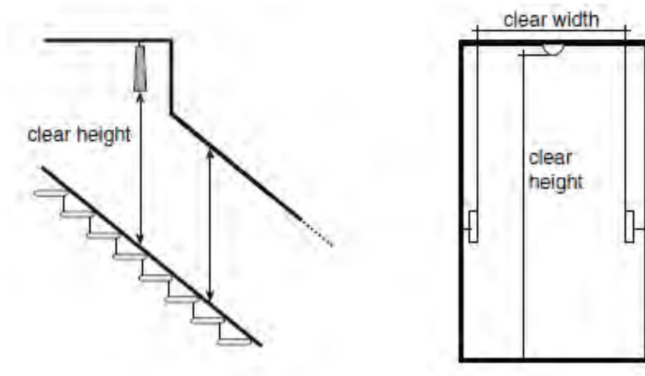
Figure A-3.4.3.4. Measuring Clear Height
