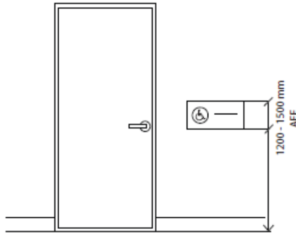
Figure A-3.8.3.1.(5) Height of Accessibility Signs
