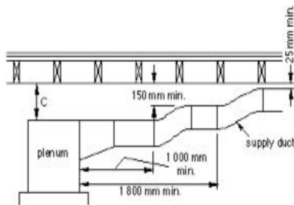
Figure A-6.2.4.10.(3) Applicable to forced-air furnaces where permissible clearance C above plenum is more than 150 mm.
