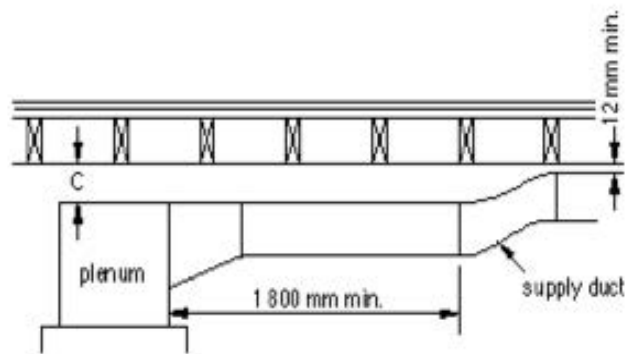
Figure A-6.2.4.10.(2) Applicable to forced-air furnaces where permissible clearance C above plenum is more than 75 mm but not more than 150 mm.
