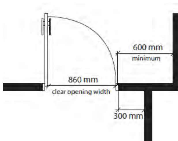
Figure A-3.8.3.3.(1) Clear Doorway Width
