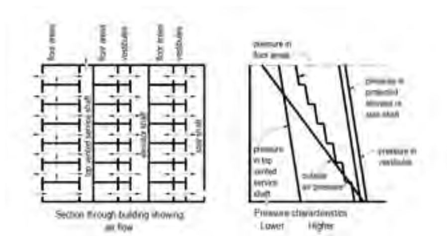
Figure 22 Pressure characteristics in a Measure D building having air injected into vestibules
