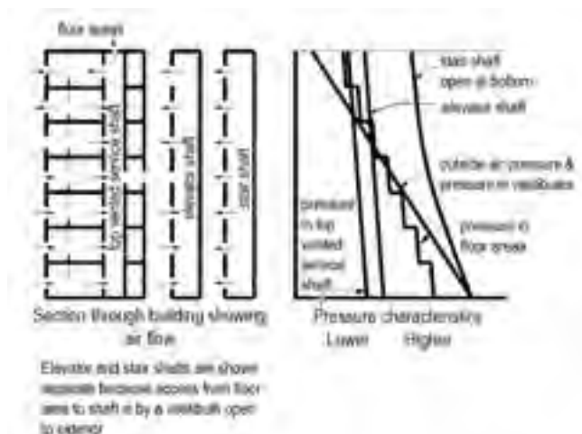
Figure 21 Pressure characteristics in a Measure D building with vented shafts
