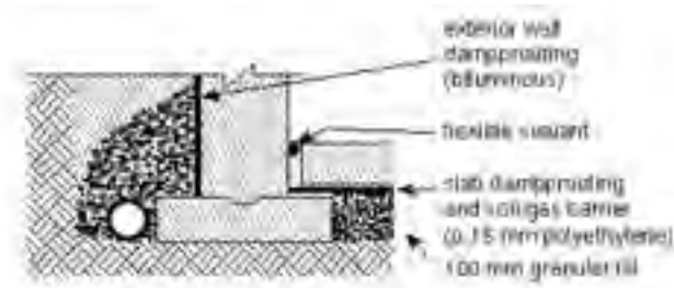
Figure SB-9A Dampproofing and Soil Gas Control at Foundation Wall/Floor Junctions with Solid Walls
