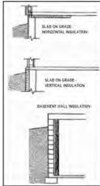
Figure 5-1 Continuity of Insulation on or Below Grade
