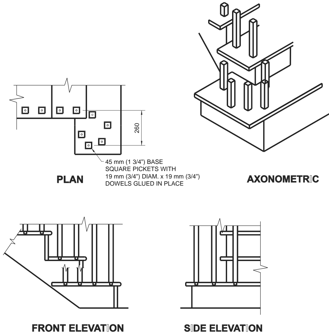
Detail IG-5
