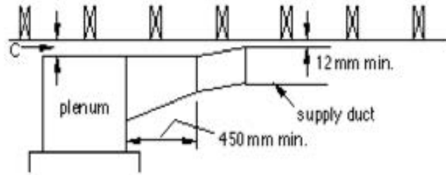
Figure A-6.2.4.10.(1) Applicable to forced-air furnaces where permissible clearance C above plenum is 75 mm or less.
