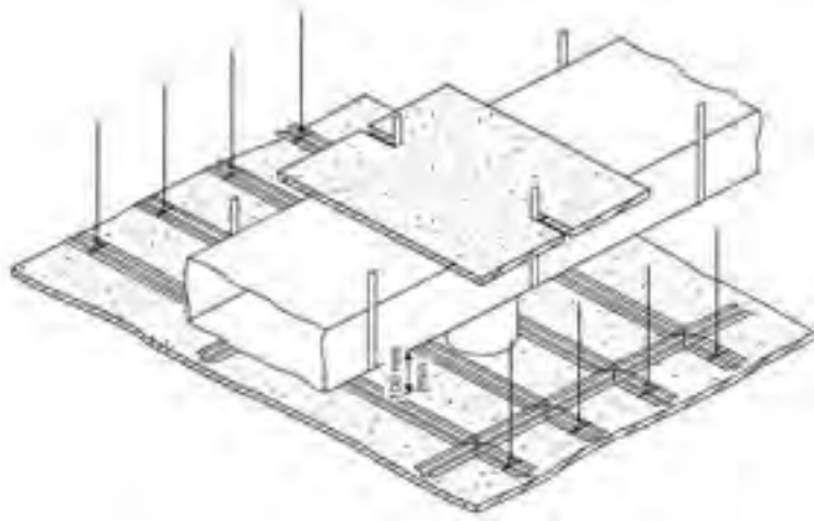
Figure 2.3.10. Thermal Protection Above a Duct
