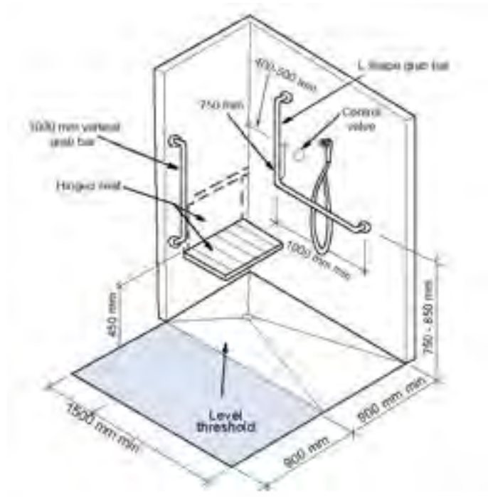
a11 Figure A-3.8.3.13.(2)(e), (f) and (g) Accessible Shower
